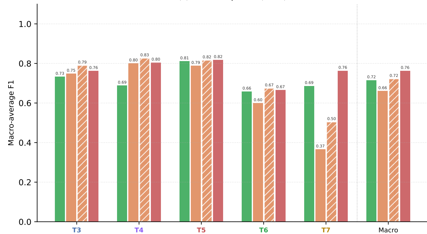
(b) Model comparison (T3-T7)
