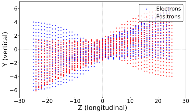
Figure 2: Beam-beam collision calculated by the AI-generated code. Arbitrary units. Electrons are moving right.
