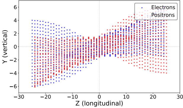
Figure 2: Beam-beam collision calculated by the AI-generated code. Arbitrary units. Electrons are moving right.
