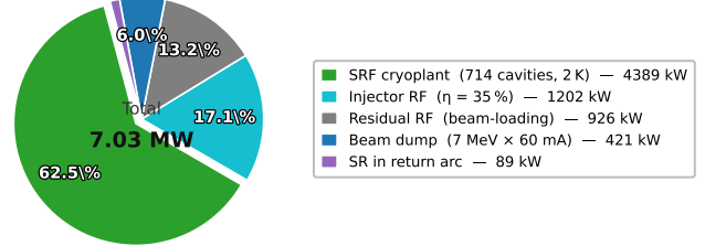
Figure 5: Single-pass ERL wall-plug power budget (10 GeV, 60 mA, f_{RF} = 801.58 MHz) produced by vibe-coding.
