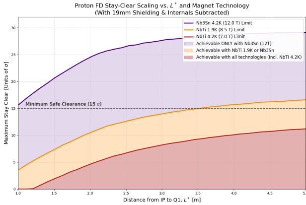
Figure 4: Hybrid EIC-LHeC FD stay-clear vs L^* and SC magnet technology analyzed via vibe-coding.
