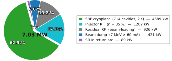
Figure 5: Single-pass ERL wall-plug power budget breakdown produced by vibe-coding with Claude.
