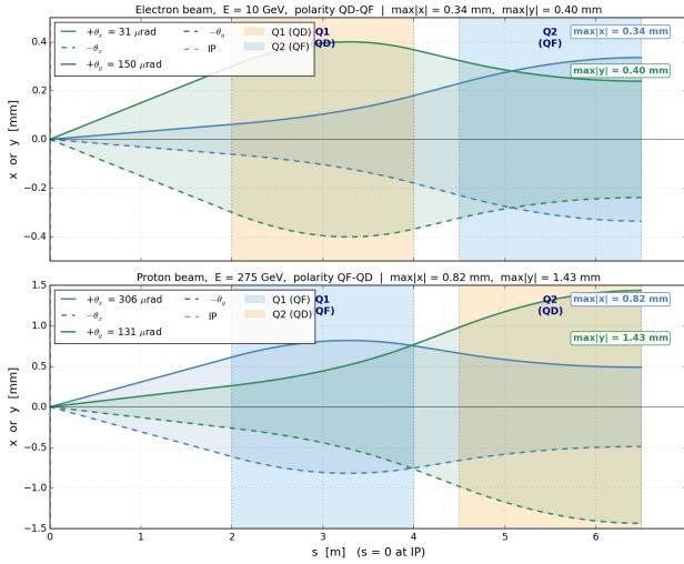
Figure 3: Hybrid EIC-LHeC FD produced via vibe-coding.
