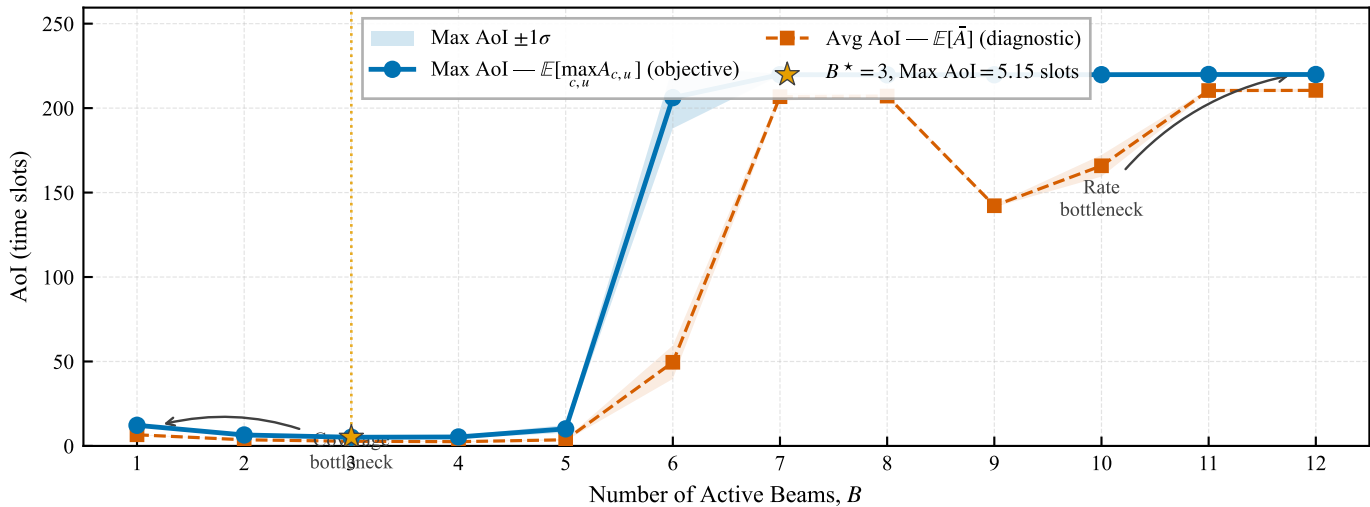
Max and Average AoI vs. B ( C=12 , K=4/\text{cell} , W_{\text{total}}=20 MHz, R_{\text{th}}=16 Mbps, Greedy)
