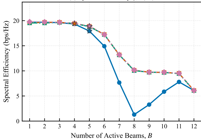
(b) Spectral Efficiency \eta_{\text{SE}} (F4)
