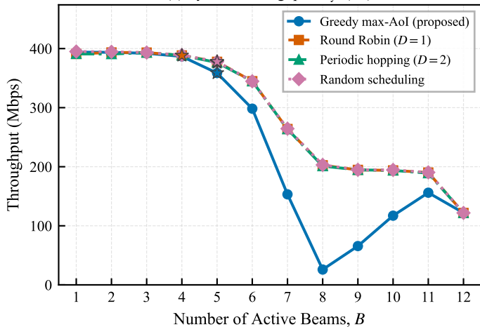
(a) System Throughput \bar{\mathcal{T}}_{\text{sys}} (F3)
