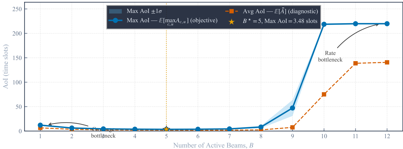
Max and Average AoI vs. B ( C = 12 , K = 4/\text{cell} , W_{\text{total}} = 20 MHz, P = 53 dBm, R_{\text{th}} = 3 Mbps)
