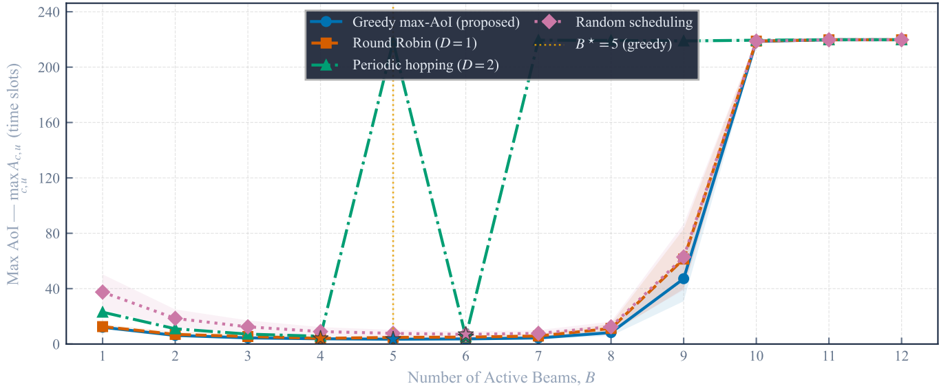
Max AoI vs. B — Four Scheduling Policies ( C = 12 , K = 4/\text{cell} , R_{\text{th}} = 3 \text{ Mbps} , T = 200 \text{ slots} )
