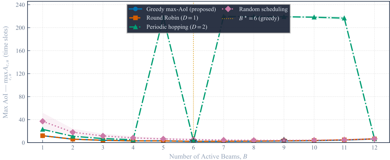
Max AoI vs. B — Four Scheduling Policies ( C=12 , K=4/\text{cell} , R_{\text{th}}=3 Mbps, T=200 slots)
