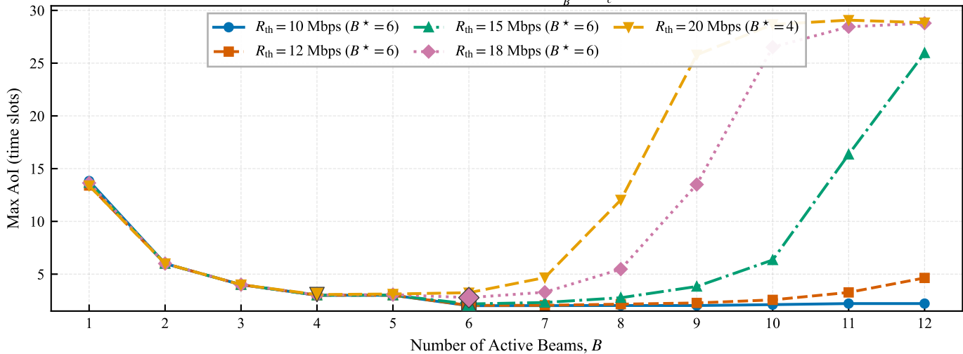
Effect of R_{th} on Optimal B^* (Objective: \min_B \mathbb{E}[\max_c A_c] , K = 1/\text{cell} )
