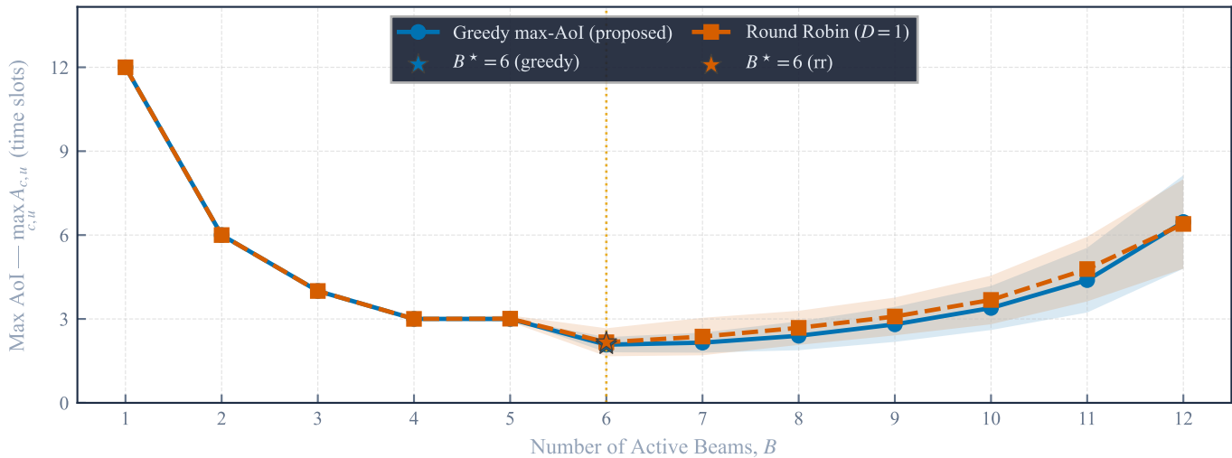
Greedy Max-AoI vs. Round Robin ( C = 12 , K = 4/\text{cell} , R_{\text{th}} = 3 Mbps)
