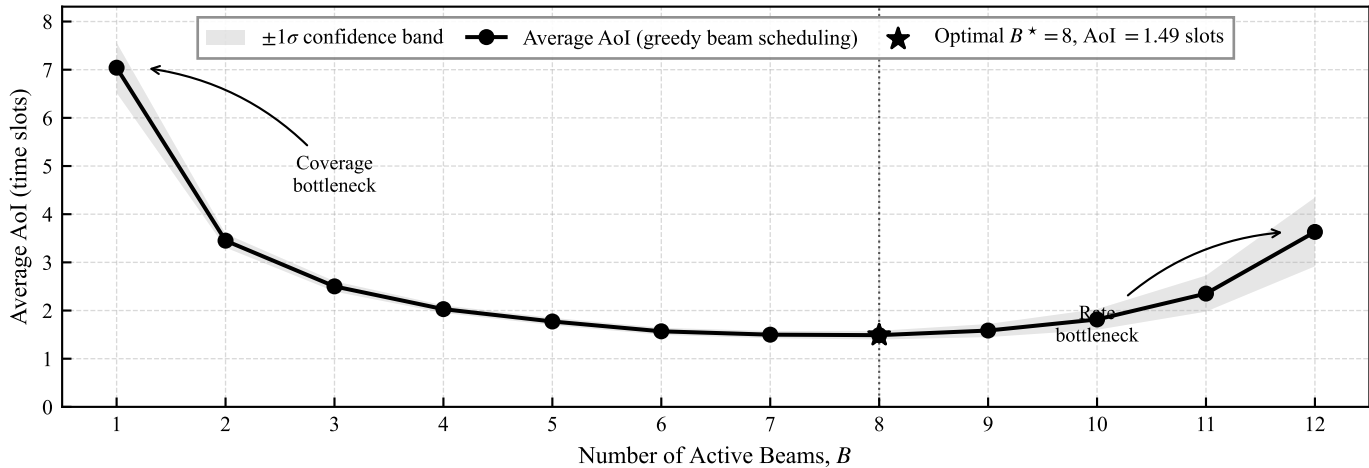
Average AoI vs. Number of Active Beams ( C = 12 , W_{\text{total}} = 20 MHz, P = 53 dBm, R_{\text{th}} = 10 Mbps)
