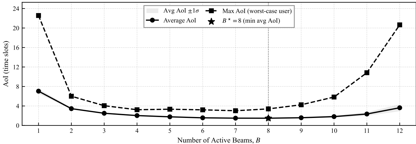
Average and Maximum AoI vs. Number of Active Beams
