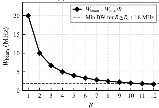
(a) Bandwidth per Beam
