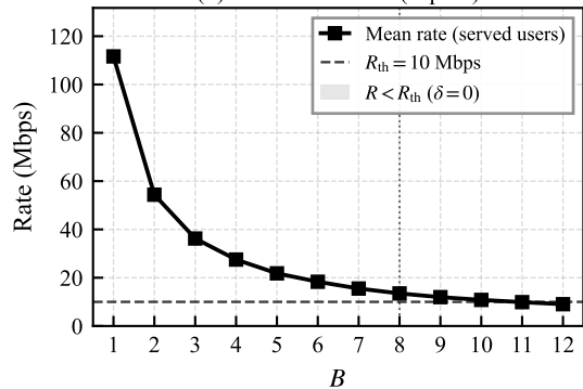
(b) Achievable Rate (Eq. 15)
