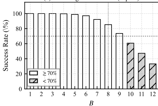
(c) Decoding Success Rate (Eq. 24)
