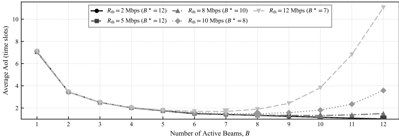
Effect of Rate Threshold R_{th} on Optimal B^*
