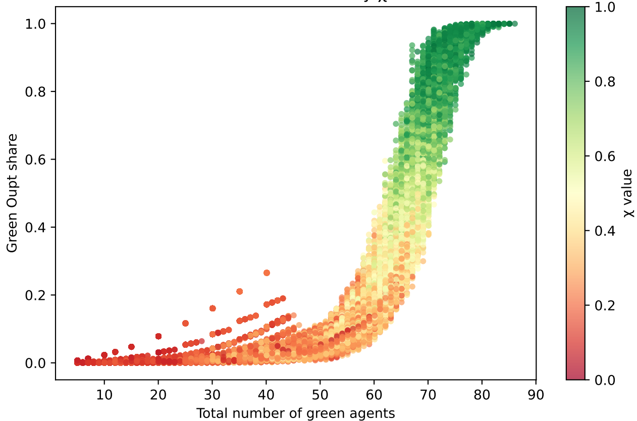
Macro variables colored by \chi value
