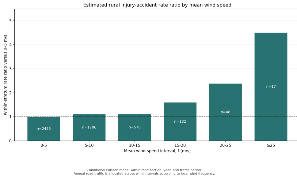
Figure A.10: Estimated rural injury-accident rate ratios relative to 0–5 m/s. The model compares wind intervals within the same road section, year, and traffic period. Traffic is allocated within a period in proportion to local 10-minute wind frequency. Labels show observed accidents.
