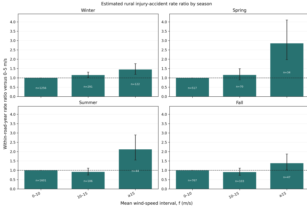
Figure 4.5: Estimated rural injury-accident rate ratios by season. Traffic and weather frequency are aligned by road section, year, and season. Coarse wind intervals avoid unstable one-event upper bins; labels show observed accidents and error bars are 95% confidence intervals.
