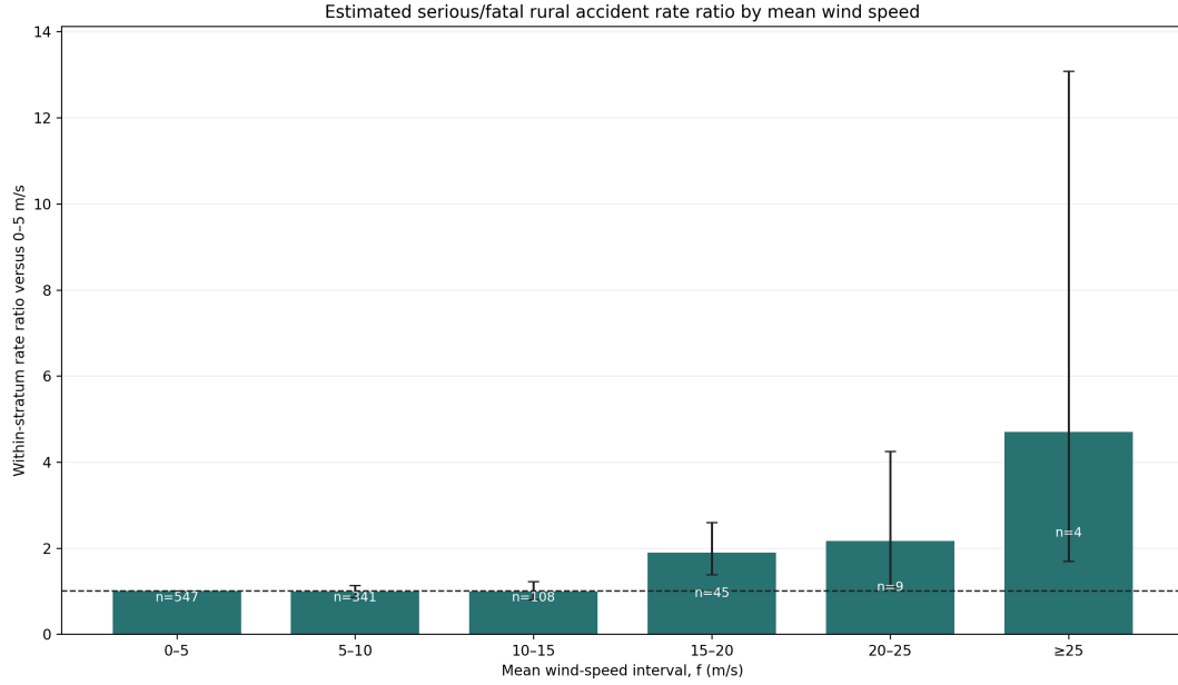
Figure 4.4: Estimated serious-or-fatal rural accident rate ratios by mean wind. The exposure and within-road-section-year-traffic-period comparison match Figure 4.3; labels show observed accidents and error bars are 95% confidence intervals.
