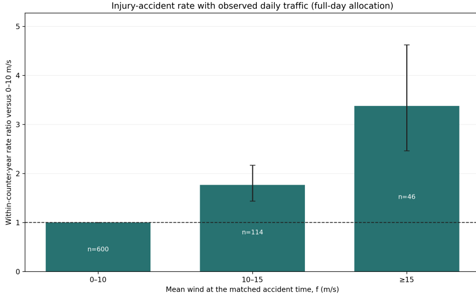
Figure 4.7: Daily-counter rural injury-accident rate ratios by accident-time mean wind. Observed 24-hour traffic is allocated within each day in proportion to the counter station’s ten-minute wind frequency. Comparisons are within counter and year; labels show accidents and error bars are 95% confidence intervals.
