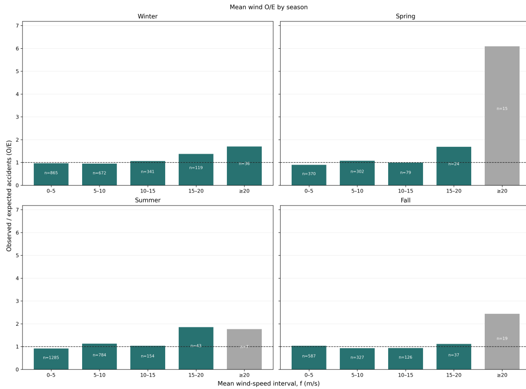
Figure A.5: Mean-wind O/E estimates by meteorological season. These estimates are shown as a descriptive subgroup analysis; high-wind bins are sparse after the sample is divided by season. All panels share one vertical scale; grey bars contain fewer than 20 accidents.
