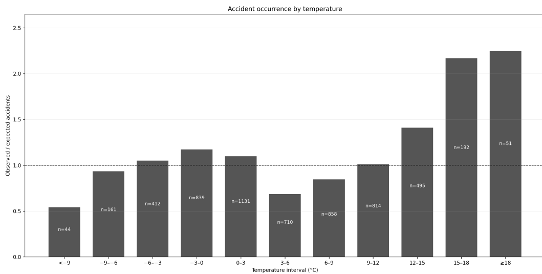
Figure A.7: Temperature O/E estimates standardised by the independently matched temperature station and meteorological season. Temperature is exploratory; mean wind remains the primary exposure. Labels give observed accident counts.
