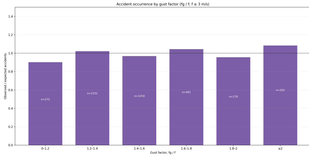
Figure A.4: Frequency-adjusted observed/expected accident occurrence by gust factor ( fg/f ). The ratio is calculated only where mean wind speed is at least 3 m/s. It does not show a clear monotonic pattern and therefore adds no evidence that gust factor alone explains the primary result. Labels show observed accidents.
