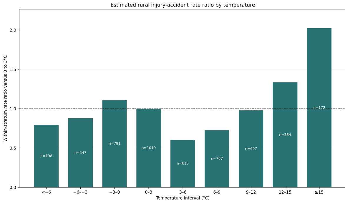
Figure 4.10: Estimated rural injury-accident rate ratios by temperature relative to 0–3°C. Comparisons are within road section, year, and traffic period. Vehicle-kilometres are allocated according to temperature frequency at the same road-assigned weather station used for the accident temperature. Labels show accidents; confidence intervals are reported in the text and result tables.
