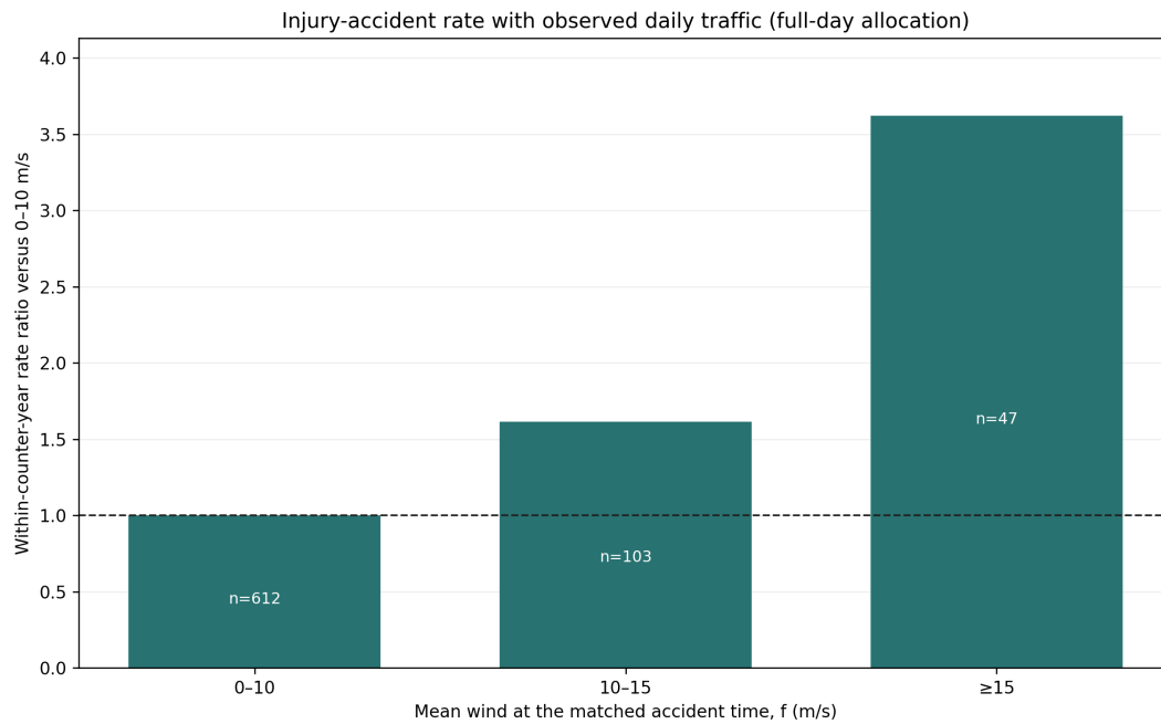
Figure 4.13: Daily-counter rural injury-accident rate ratios by accident-time mean wind. Observed 24-hour traffic is allocated within each day in proportion to the counter station's ten-minute wind frequency, and accidents use that same station. Comparisons are within counter and year; labels show accidents. Confidence intervals are reported in the text and result tables.
