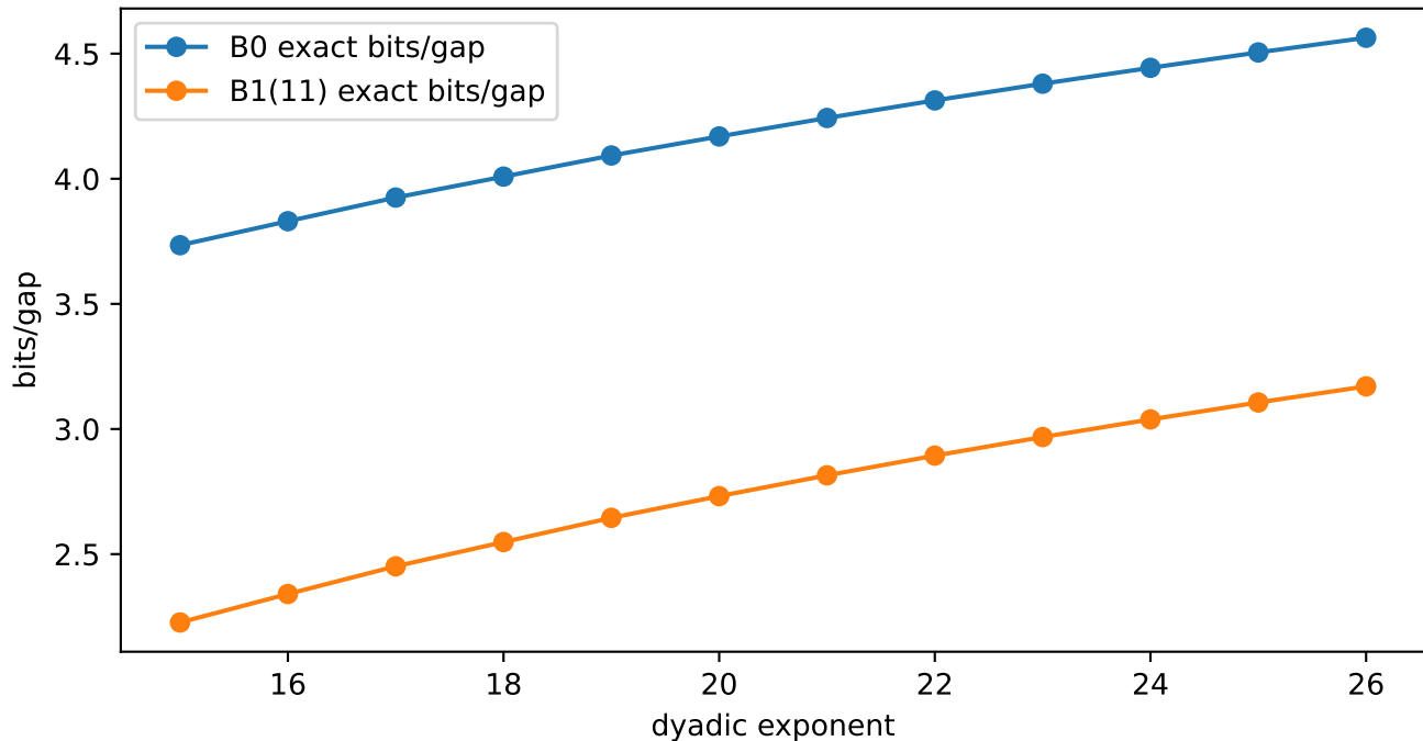
Exact baseline code lengths
