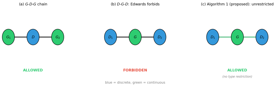
Figure 1: The D – G – D configuration that Edwards’ restriction forbids by construction. A continuous variable G lies on the path between two discrete variables D_1 and D_2 , so the factorisation requires P(D_2 \mid G) , which is not part of the standard CG parametrisation.
