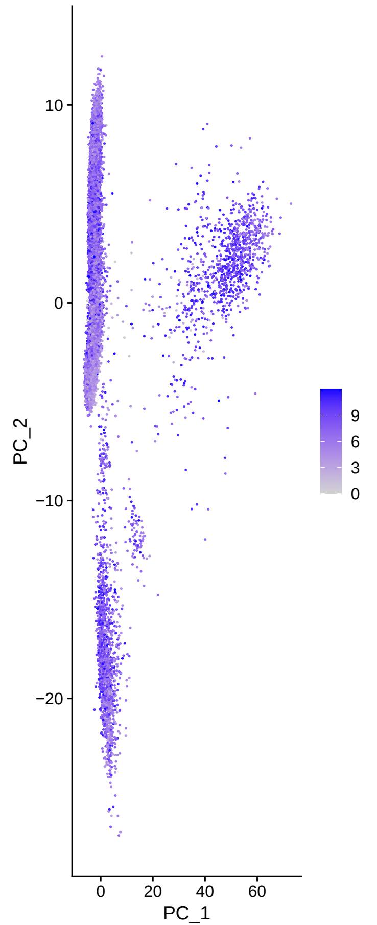
percent.mt
