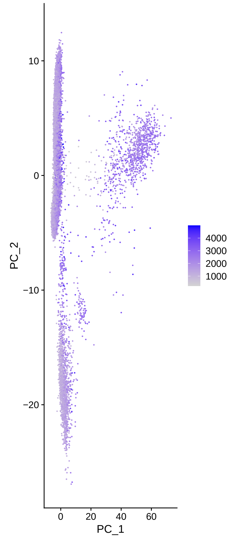
nFeature_RNA
