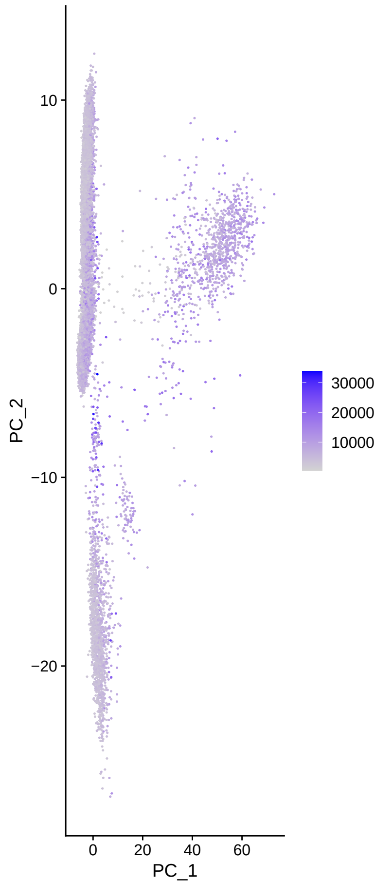
nCount_RNA
