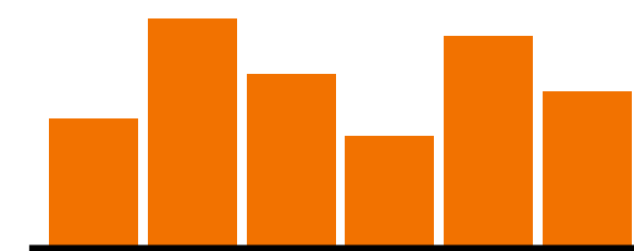
p_2(y_t | y_{<t})
