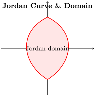
Jordan Curve & Domain
