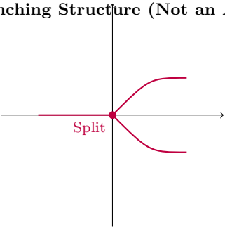
Branching Structure (Not an Arc)
