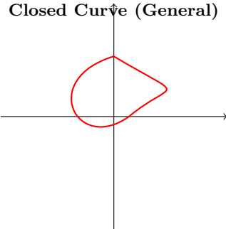
Closed Curve (General)
