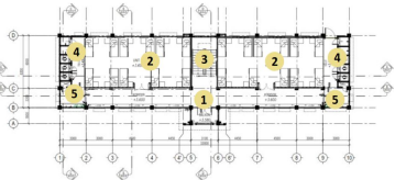
DENAH LANTAI TIPIKAL
