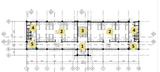
DENAH LANTAI TIPIKAL
