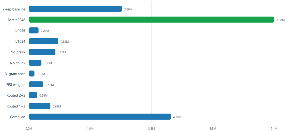
Score comparison across key runs
