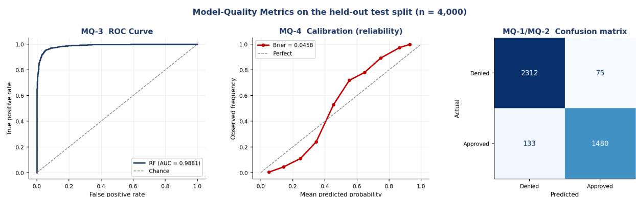
Figure 13: ROC, calibration and confusion matrix on the held-out split. The calibration curve tracking the diagonal is what makes the LOW/MEDIUM/HIGH tiering defensible — a 0.70 prediction really does correspond to roughly 70% observed approvals.
