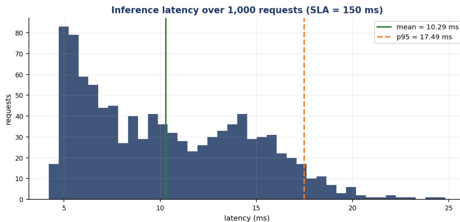
Figure 20: End-to-end scoring latency over 1,000 requests through the real serving path: mean 10.29 ms, p95 17.49 ms, p99 20.04 ms — comfortably inside the 150 ms SLA inherited from Assignment I.
