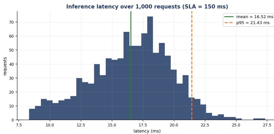
Figure 20: End-to-end scoring latency over 1,000 requests through the real serving path: mean 16.52 ms, p95 21.43 ms, p99 23.66 ms — comfortably inside the 150 ms SLA inherited from Assignment I.
