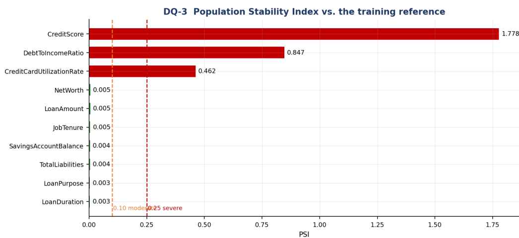
Figure 19: PSI per feature against the 0.10/0.25 industry thresholds.
