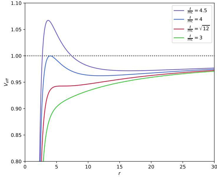
Figure 5.1: Effective potential for a massive particle moving in the Schwarzschild spacetime as function of the radial coordinate r with m = c = 1 and \ell \neq 0 . The maximum and minimum in the curves correspond to possible circular orbits (unstable and stable) around the central mass for a given value of \ell . The red curve corresponds to the extreme case \ell^2 = 12m^2c^2 for which it is possible to see the inflection point defining the Innermost Stable Circular Orbit (ISCO). Smaller angular momenta produce curves as the green one, with no maxima, minima or inflection points and therefore, no circular motion.
