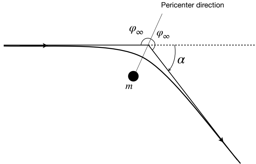
Figure 5.3: The deflection angle \alpha from a light-ray moving in Schwarzschild's spacetime. The incident and scattered rays have directions given by the angle \varphi_\infty with respect to the direction of the perihelion.
