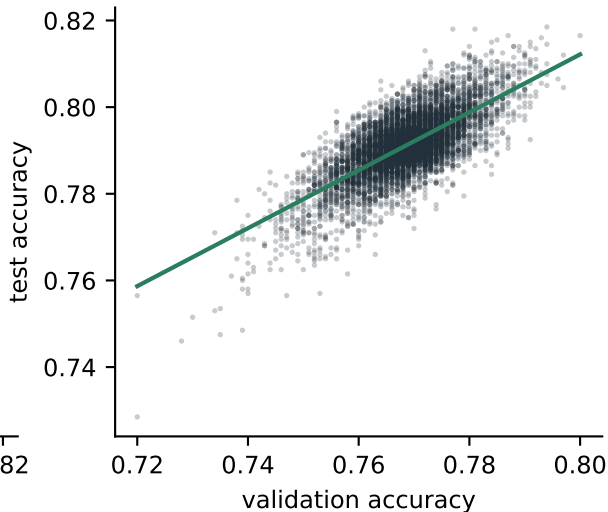
(b) selection transfers ( r = 0.72 )
