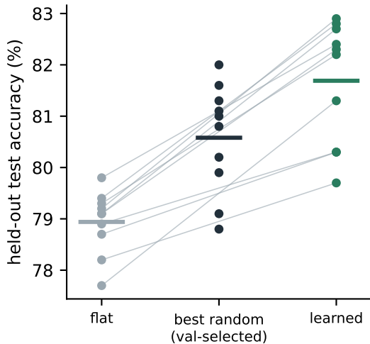
(b) ten held-out seeds
