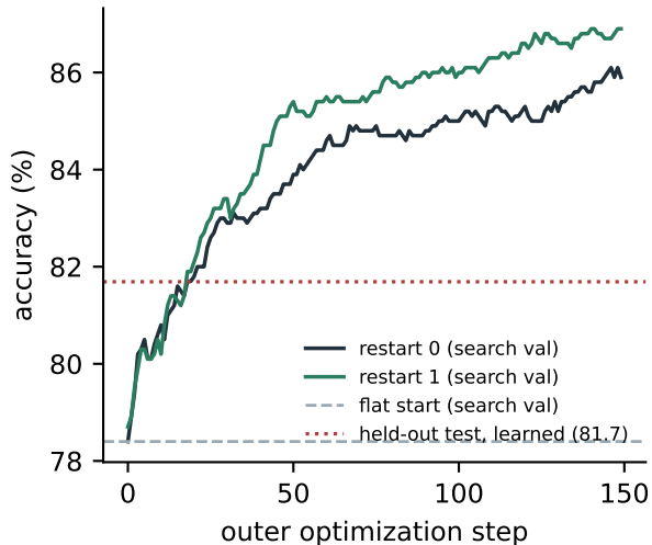
(a) search curves vs the held-out result
