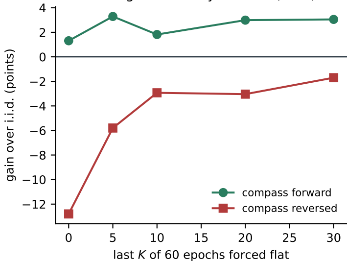
Closing the recency channel (Cora)
