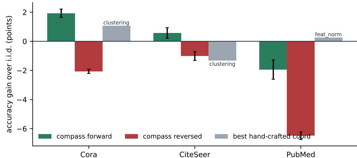
Path effect replicates in direction; exploitability decays with graph size
