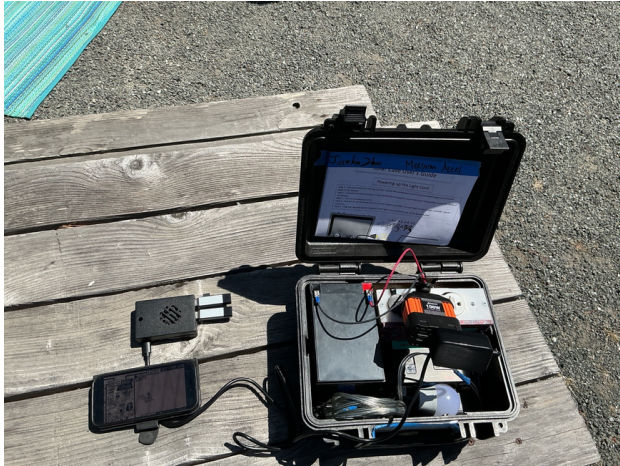
VILLAGESERVER CASE WITH USB READERS
