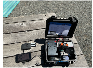
VILLAGESERVER CASE WITH USB READERS
