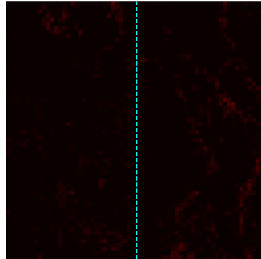
|Diff| hard partition (mean=0.006)
