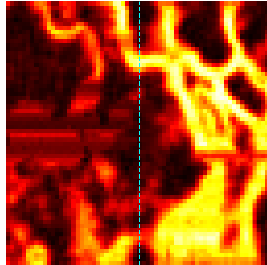
|Diff| naive sum (mean=0.333)
