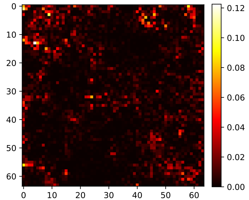
Diff Axial
