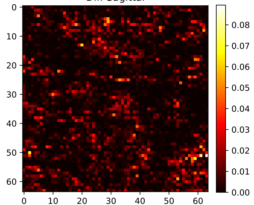
Diff Sagittal
