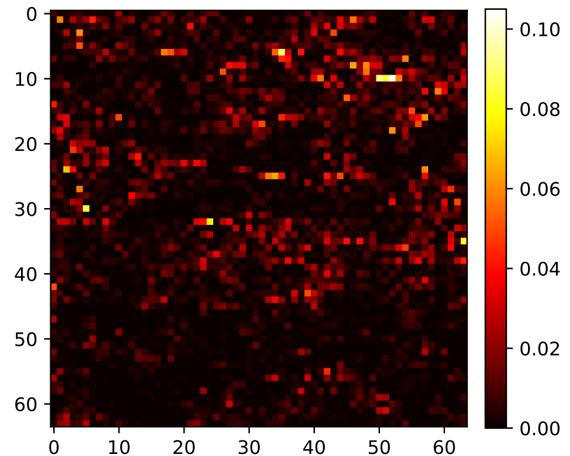
Diff Coronal
