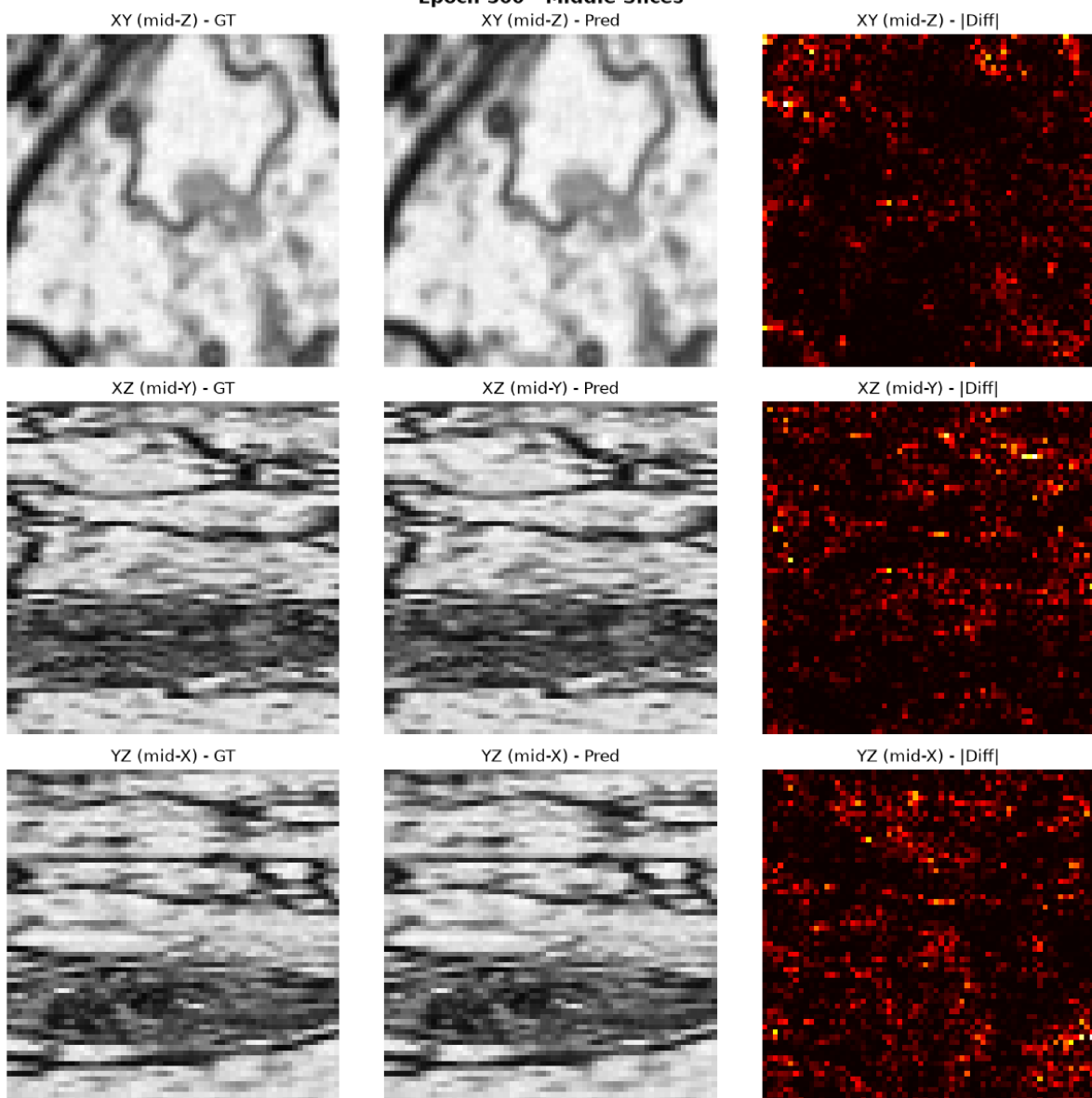
(c) b_221 — vol_PSNR = 40.38 dB
