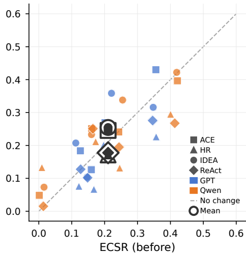
Procedural induction
