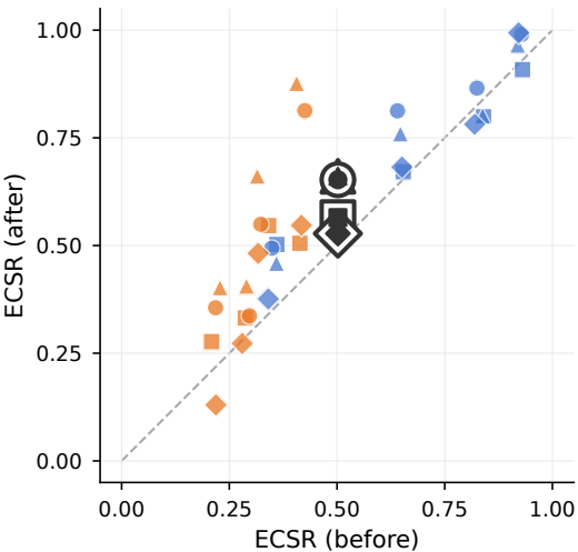
Attribute induction
