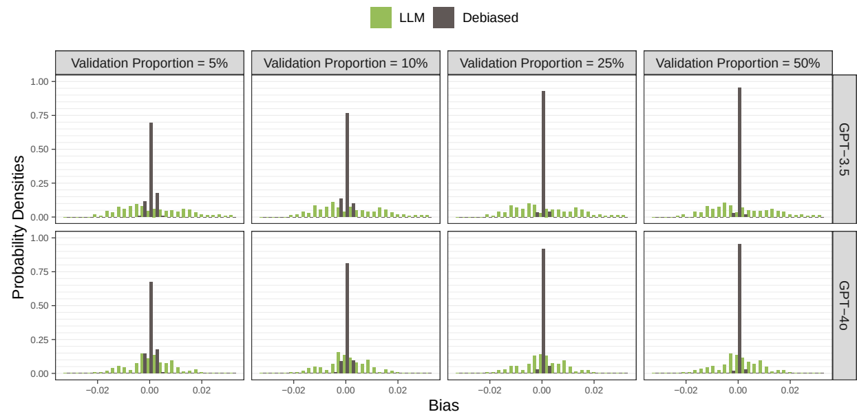
Figure 5: Bias Density of \beta by Model and Proportion of Validation Samples. Proxy on the LHS.
