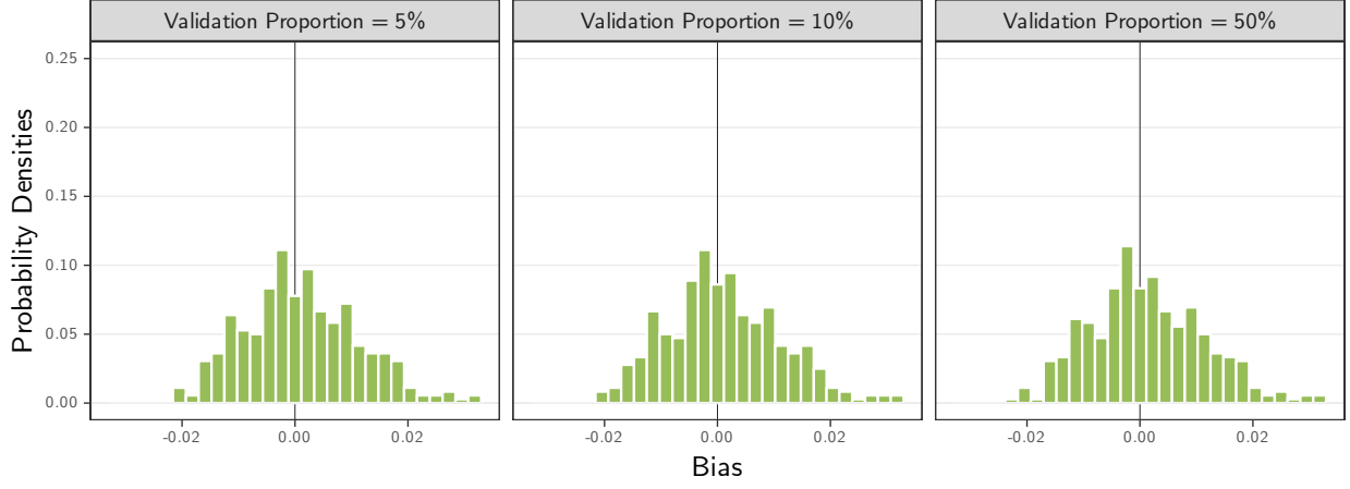
Figure 4: Bias Density of \beta_1^{\text{LLM}} by Proportion of Validation Samples. Proxy on the LHS.
