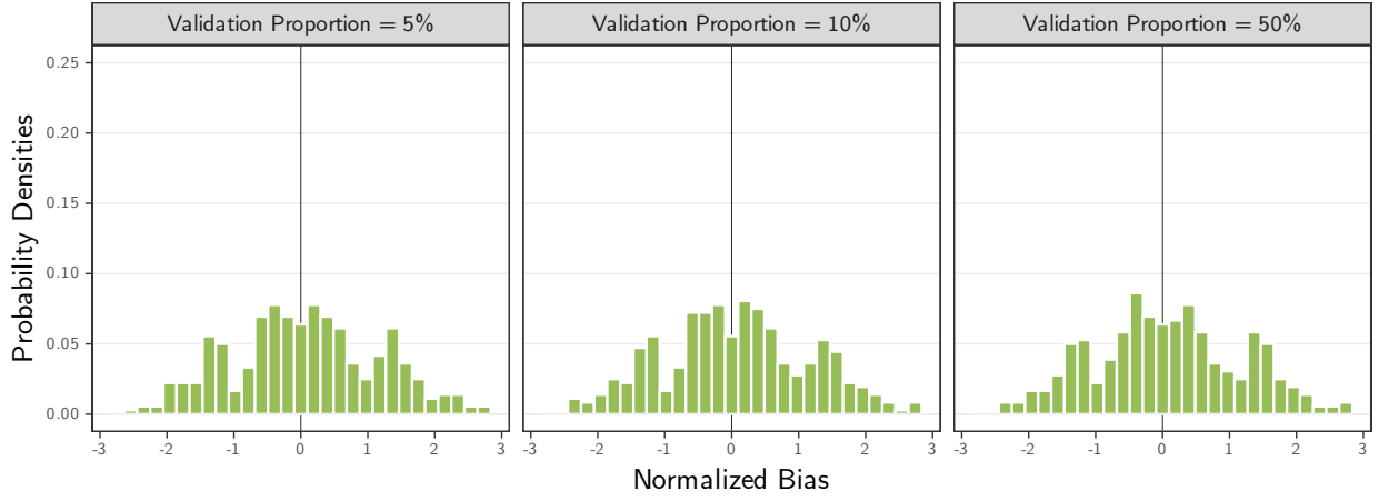
Figure 5: Normalized Bias Density of \beta_1^{\text{LLM}} by Proportion of Validation Samples. Proxy on the LHS.
