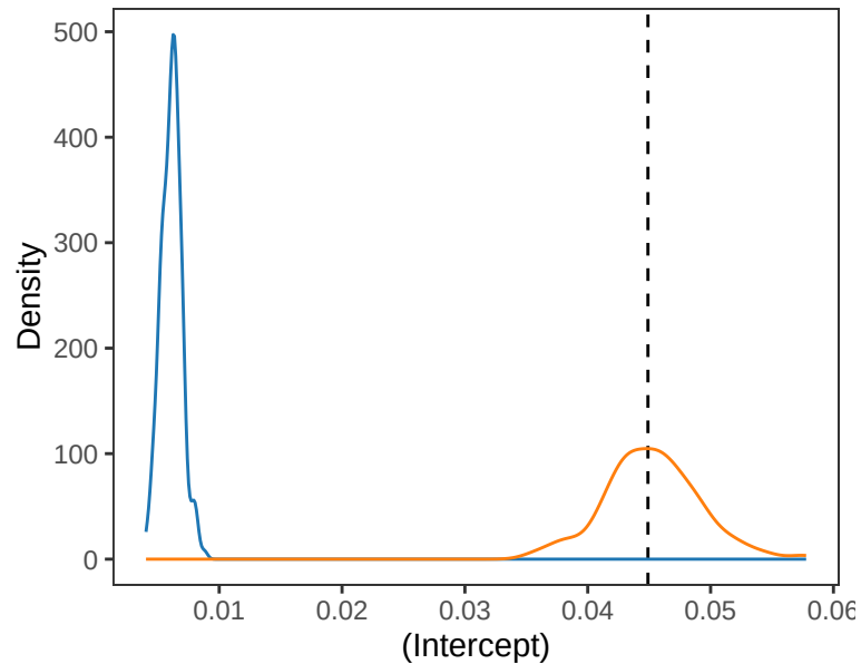
Density Plot for (Intercept)
