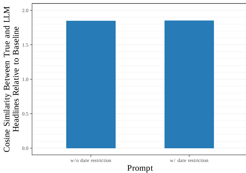
Figure 1: Cosine Similarity Between True and LLM Headlines Compared to a Random Baseline, GPT-4o, by Prompt
