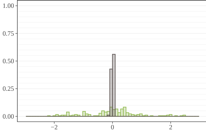
GPT-5-Mini
