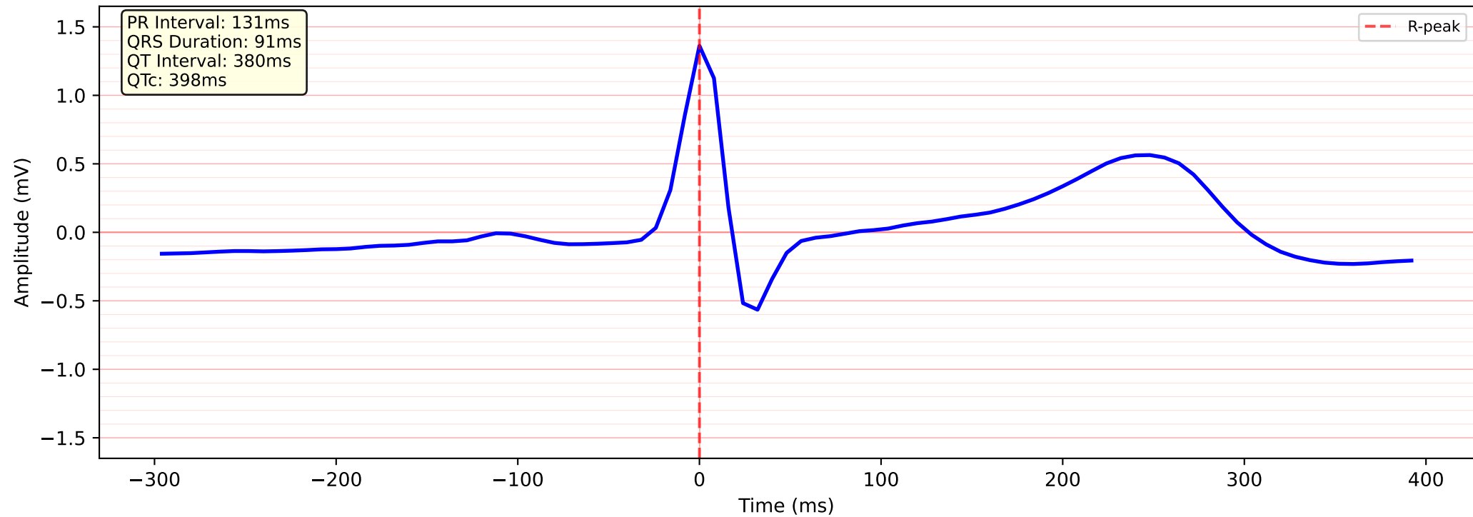
Single Beat Detail
