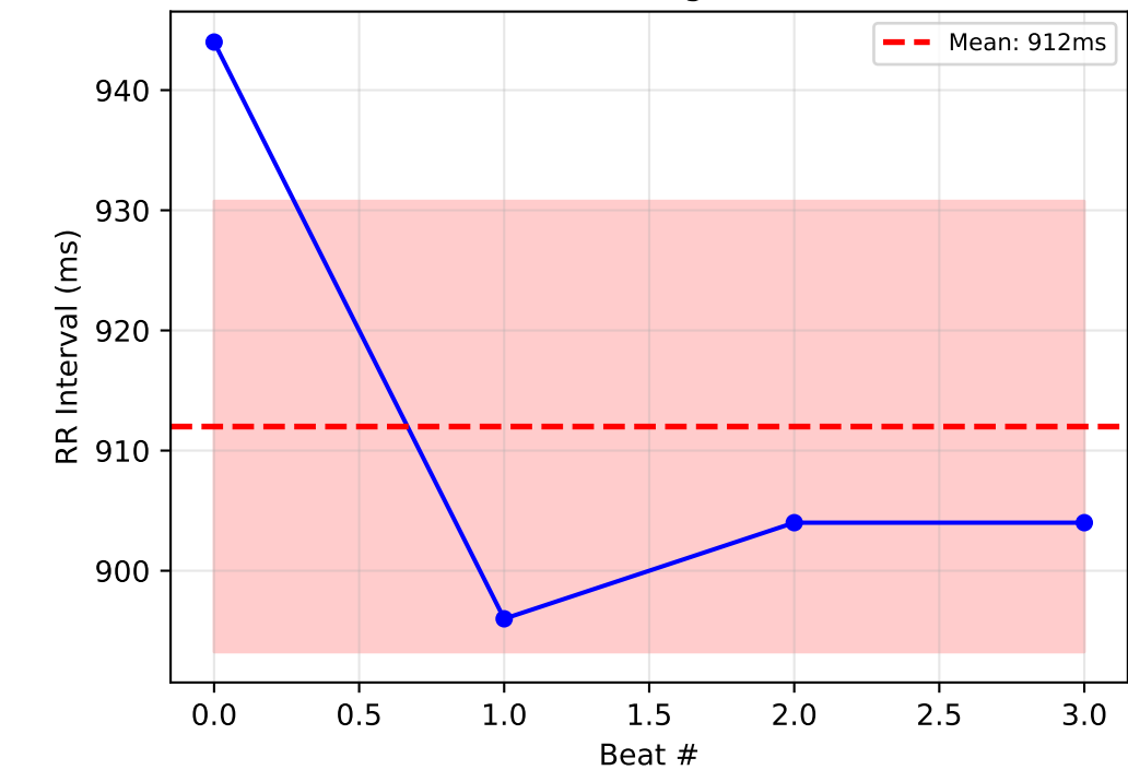
RR Tachogram
