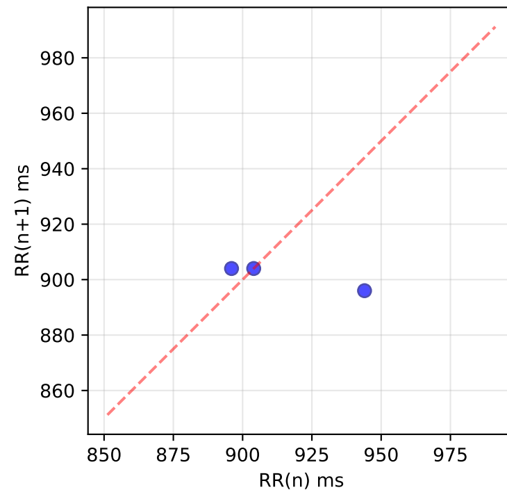
Poincaré Plot
